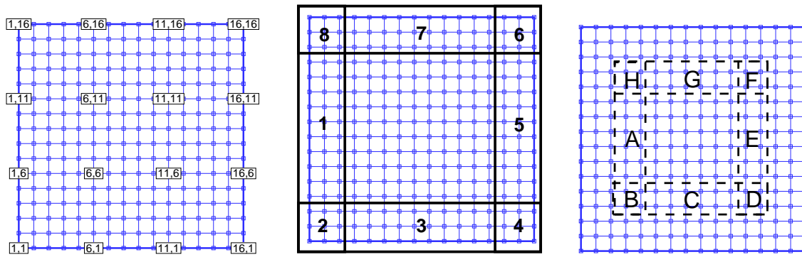
Figure 3: (Left) Typical WENO subdomain. (Middle) "Ghost Area". (Right) "Buffer Area".
