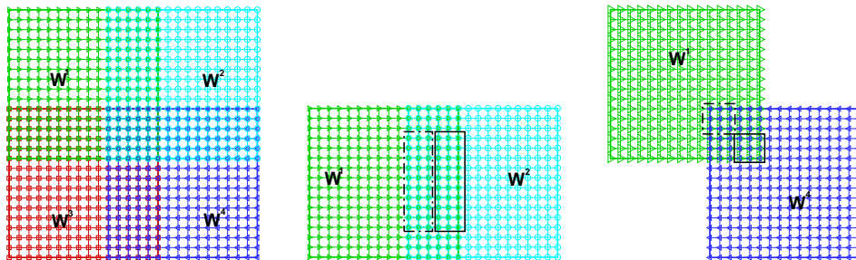
Figure 5: (Left) WENO-WENO-WENO-WENO subdomain configuration. (Middle) W^1 - W^2 Interface. (Right) W^1 - W^4 Interface.
