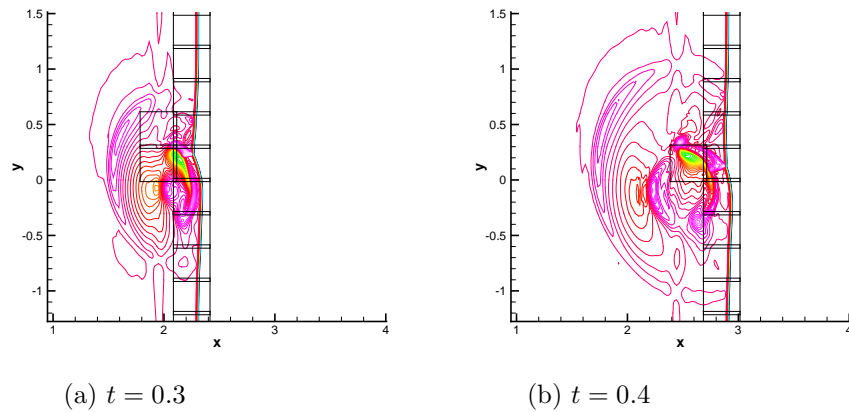
Figure 10: Density \rho of the Shock-Vortex interaction with Mach number M_s = 6 and \Gamma = 0.25 at time (a) t = 0.3 and (b) t = 0.4 as computed by the Hybrid method.
