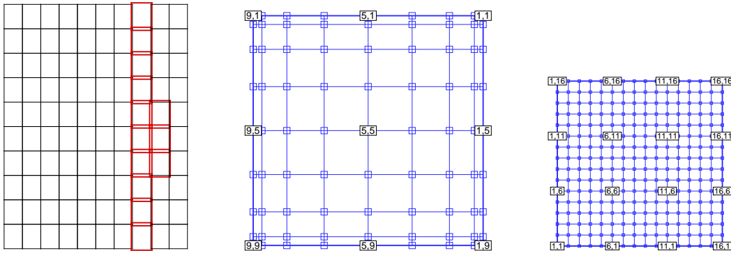
Figure 2: (Left) Partition of the physical domain into spectral and WENO subdomains. (Middle) Typical spectral subdomain. (Right) Typical WENO subdomain.
