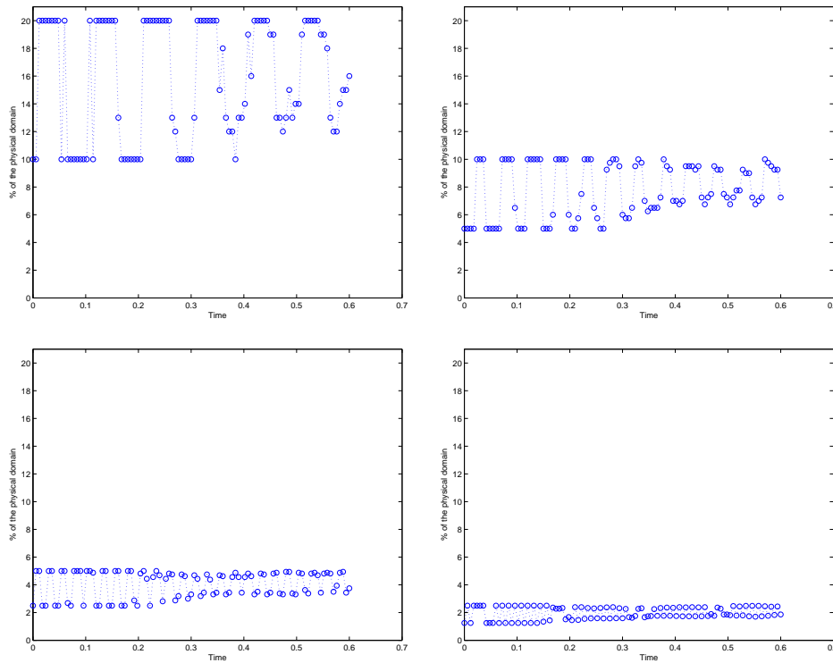
Figure 15: The time history of the coverage of the WENO subdomains as a percentage of total number of subdomains for the four subdomain partitions. Top: 10 \times 10 and 20 \times 20 ; Bottom: 40 \times 40 and 80 \times 80 .
