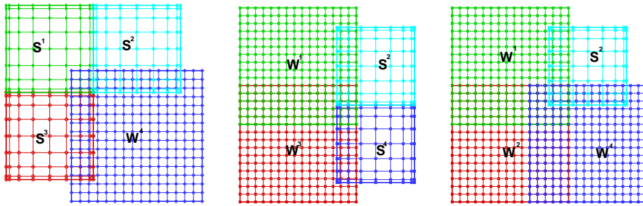
Figure 6: Subdomain Configurations: (Left) Spectral-Spectral-Spectral-WENO. (Middle) Spectral-Spectral-WENO-WENO. (Right) Spectral-WENO-WENO-WENO.
