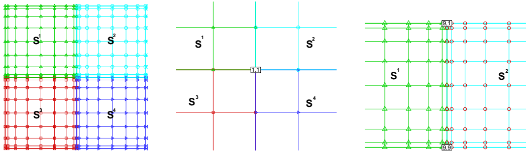
Figure 4: (Left) Spectral-Spectral-Spectral-Spectral subdomains configuration. (Middle) Corner point of all four spectral subdomains. (Right) Shared side of two spectral subdomains.
