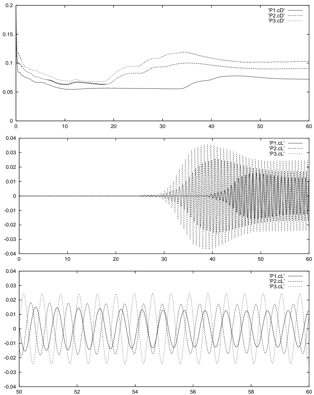
Figure 16: NACA 0012 profile ( M=0.85 , \alpha=0^\circ , Re=10000 ), dependence of the drag (up) and lift (middle and detail down) coefficients on time computed by the BDF-DGFE method with piecewise linear (P1), quadratic (P2) and cubic (P3) approximation in space and third order in time.
