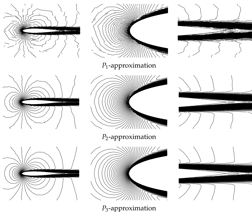
Figure 15: NACA 0012 profile ( M=0.5 , \alpha=0^\circ , Re=5000 ), isolines of the Mach number (left) with details around the leading (middle) and trailing edges (right) computed by P_1 , P_2 and P_3 approximations.
