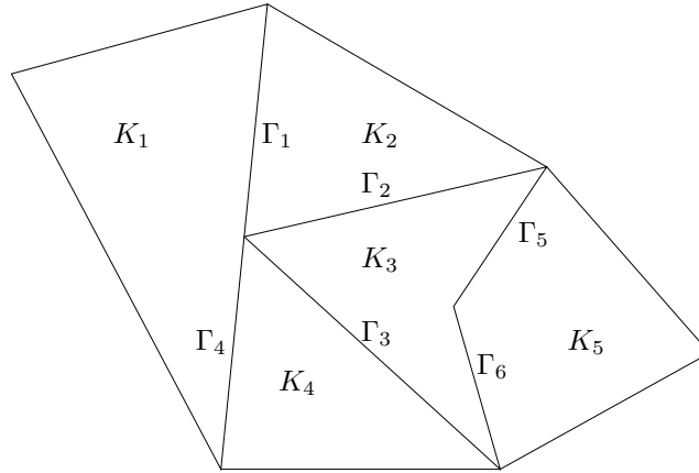
Figure 1: Example of elements K_l , l=1, \dots, 5 and faces \Gamma_l , l=1, \dots, 6 with the corresponding \mathbf{n}_{\Gamma_l} .
