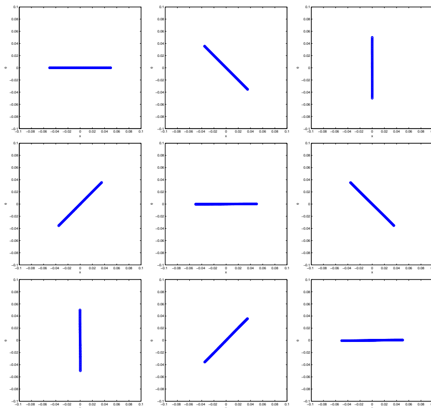
Figure 14: Diffraction of a Gaussian in a parabolic medium. We show the evolution of the open level curve in the x - \theta phase space. Caustics are clearly observed at the third and the seventh subplot.
