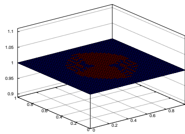
(b) n (classical scheme)
