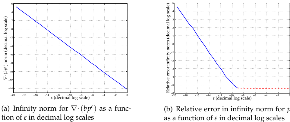
Figure 2: Oblique magnetic field test case for \alpha = \pi/3 and \Delta x = \Delta y = 1/60 . Approximation of the p^\epsilon part of the solution.
