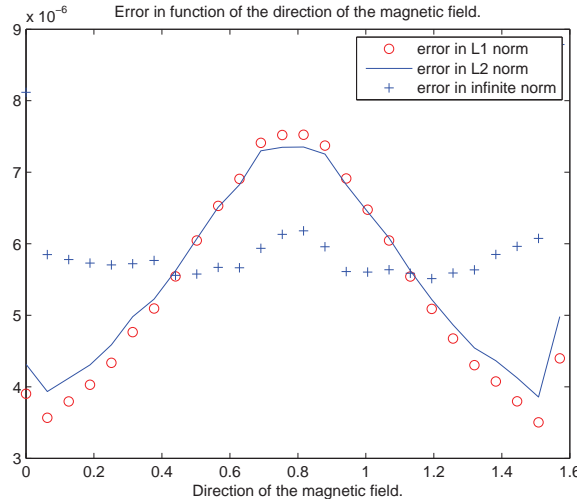
Figure 3: Oblique magnetic field test case for \varepsilon=10^{-9} and \Delta x=\Delta y=1/40 . Norms of the relative error (4.1) as a function of the angle of the magnetic field with the x -axis \alpha .
