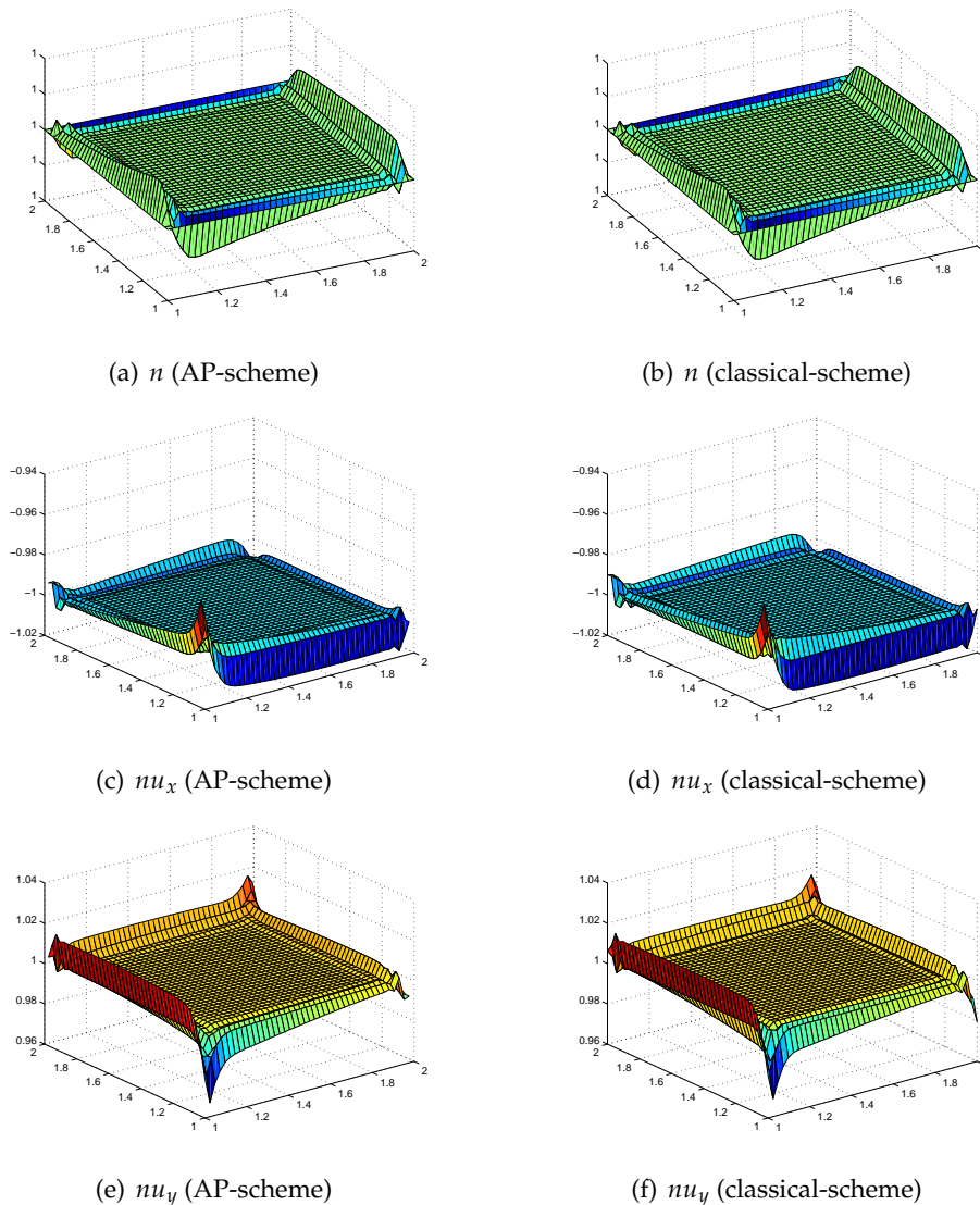
Figure 7: Euler-Lorentz test case for a non uniform magnetic field in the resolved case at time t = 3.9510^{-6} s: density ( n ) and momentum ( nu_x , nu_y ) computed by the AP-scheme (left) and the classical scheme (right) for \epsilon = 10^{-9} and \Delta x = \Delta y = 1/40 .
