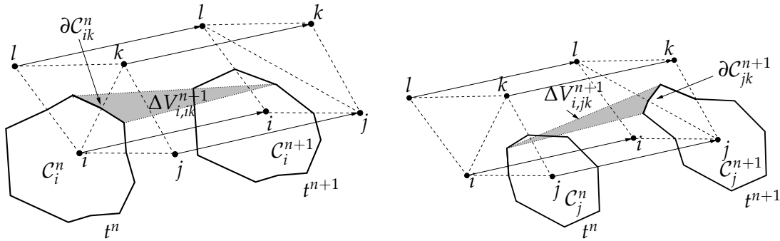
Figure 3: Interpretation of the edge swapping as continuous finite volume deformation. Left: evaluation of the normal interface velocity (area of the shaded region) for edge i - k that is deleted due to edge-swapping from edge i - k at time t^n into edge j - k at time t^{n+1} . Right: evaluation of the normal interface velocity for edge j - k that is created due to edge-swapping.
