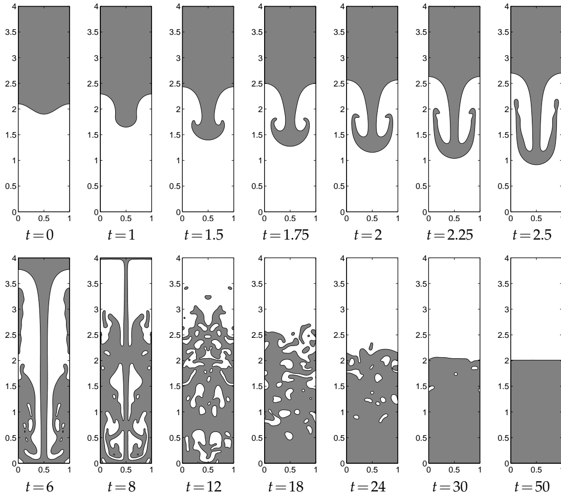
Figure 18: Long time evolution of the Rayleigh-Taylor instability simulation with At=0.5 . The dimensionless times are shown below each figure.
