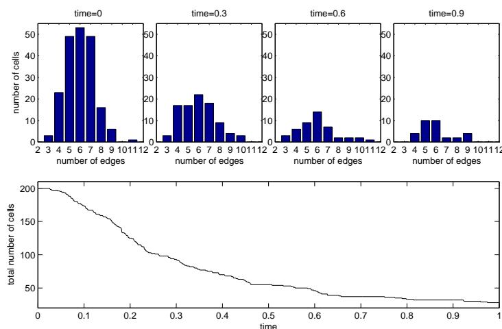
Figure 11: Results from the simulation shown in Fig. 10. Upper panels show the numbers of bubbles with different numbers of edges at selected times, and the lower panel shows the total number of bubbles as a function of time.
