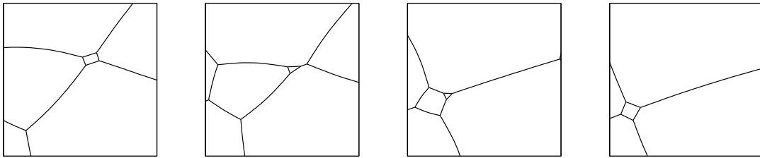
Figure 3: The effect of T1 and T2 processes. The T1 process between the 1st and the 2nd panels reduces by one the number of edges of two bubbles including the 4-edged bubble and increases by one the number of edges of two other bubbles. Then the 3-edged bubble shrinks further and disappears by the T2 process in the 4th panel.
