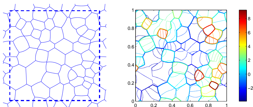
Figure 5: Initial configuration: the ‘relaxed’ configuration of a foam (left) obtained from the Voronoi network shown in Fig. 4 and the corresponding pressure contours (right). The dashed line in the left panel represents the periodic unit square. Note that bubble boundaries are not explicitly drawn in the right panel. They are visible anyway because the steep pressure gradient across the bubble boundaries makes the pressure contours concentrate along those boundaries.
