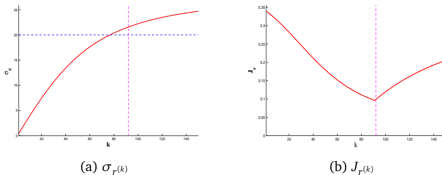
Figure 4: Standard deviation (a) and auto-correlation energy (b) of the residue.
