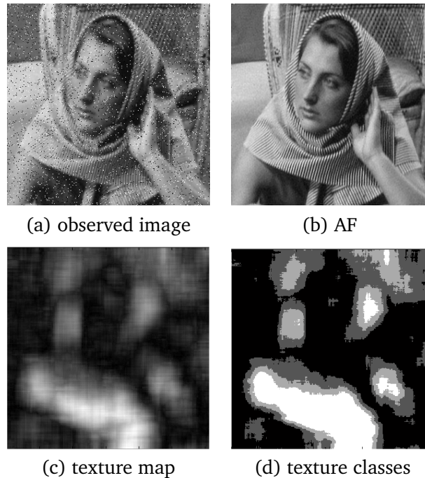
Figure 8: Example 6.2. barbara images: (a) the corrupted image produced by Gaussian blur, defined by the parameters \text{band} = 3 and \text{sigma} = 1.5 and by 5% salt & pepper additive noise; (b) restored image determined by AF algorithm; (c) texture map computed on (a); (d) texture classes from (c).
