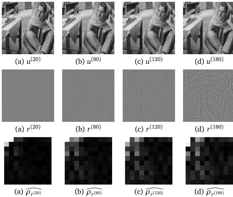
Figure 3: Some steps of the TV-flow applied to the Barbara image corrupted by a white Gaussian noise with \sigma = 20 (first row); corresponding residual images (second row); corresponding sample auto-correlation, restricted to the smaller lags [l, m] : l, m = 0, 1, \dots, 9 (third row).
