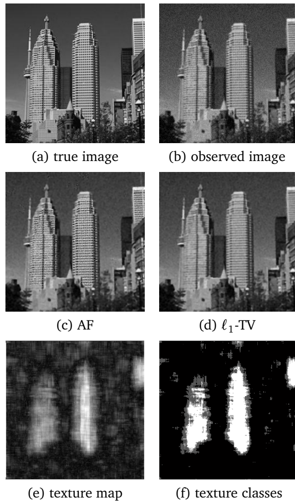
Figure 9: Example 6.3. skyscraper images: (a) original unperturbed image (b) corrupted image produced by Gaussian blur, defined by the parameters \text{band} = 3 and \text{sigma} = 1.5 and by 10% Gaussian additive noise; (c) restored image determined by AF algorithm; (d) restoration with \ell_1 -TV with \lambda_1 = 0.5 ; (e) texture map computed on (b); (f) texture classes computed on (e).
