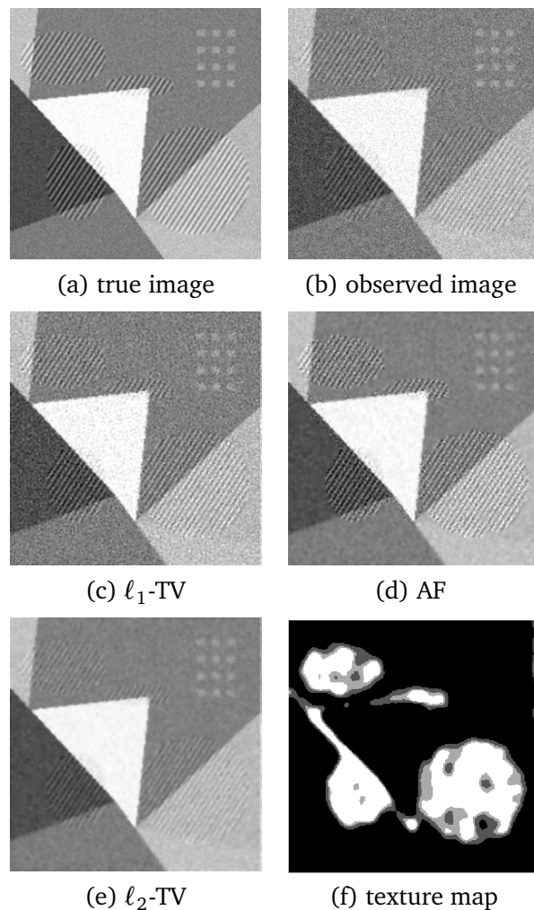
Figure 6: Example 6.1. test images: (a) blur- and noise-free image; (b) the corrupted image produced by Gaussian blur, defined by the parameters \text{band} = 3 and \text{sigma} = 1.5 and by 10% of Gaussian noise; (c) restoration with \ell_1 -TV with \lambda_1 = 0.1 ; (d) restored image determined by AF algorithm; (e) restoration with \ell_2 -TV with \lambda_1 = 0.1 ; (f) texture classes computed on (b).
