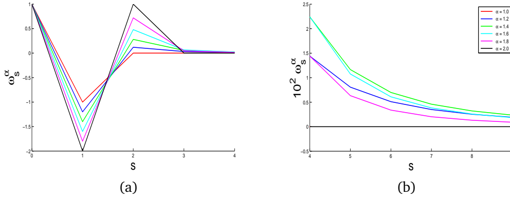
Figure 2: Values of the coefficients \omega_s^\alpha used in (4.1) for the discrete approximation of the fractional-order partial derivatives.
