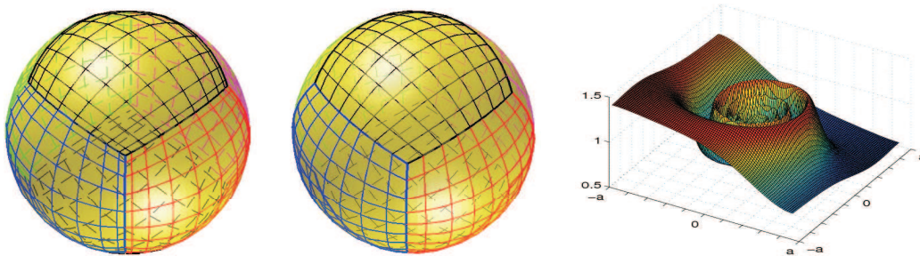
Figure 5: The grid distribution on the sphere with 10 \times 10 points on each patch. Left: LGL points. Middle: prolate points with c=8 . Right: Vortex near the north pole simulated by the prolate-element method with a third-order Adams-Bashforth time marching scheme.
