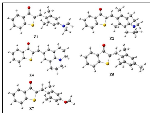
Figure 1: The optimized ground-state geometries in DCM at the PCM/CAM-B3LYP/6-31+g(d, p) calculation level.
