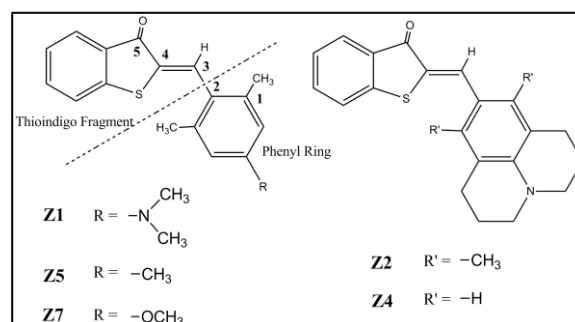
Figure 1. The chemical structures of Hemithioindigo Z1, Z2, Z4, Z5 and Z7.
